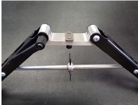
The Sudami F-Tr Bipod
